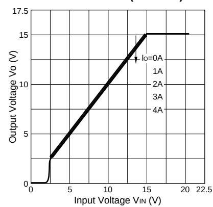
Rise Characteristics(STR9015)
