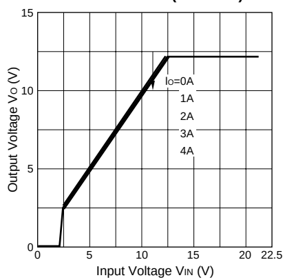
Rise Characteristics(STR9012)
