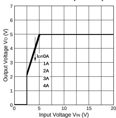
Rise Characteristics(STR9005)
