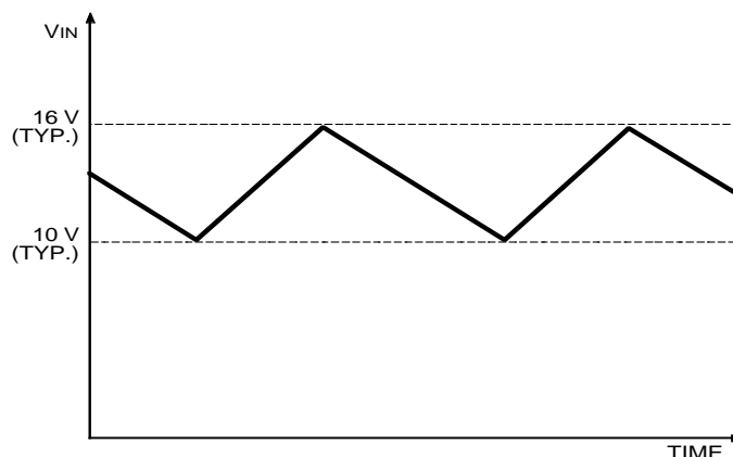
Figure 9 – Example of V_{IN} Terminal Voltage Waveform at Latch Circuit On
