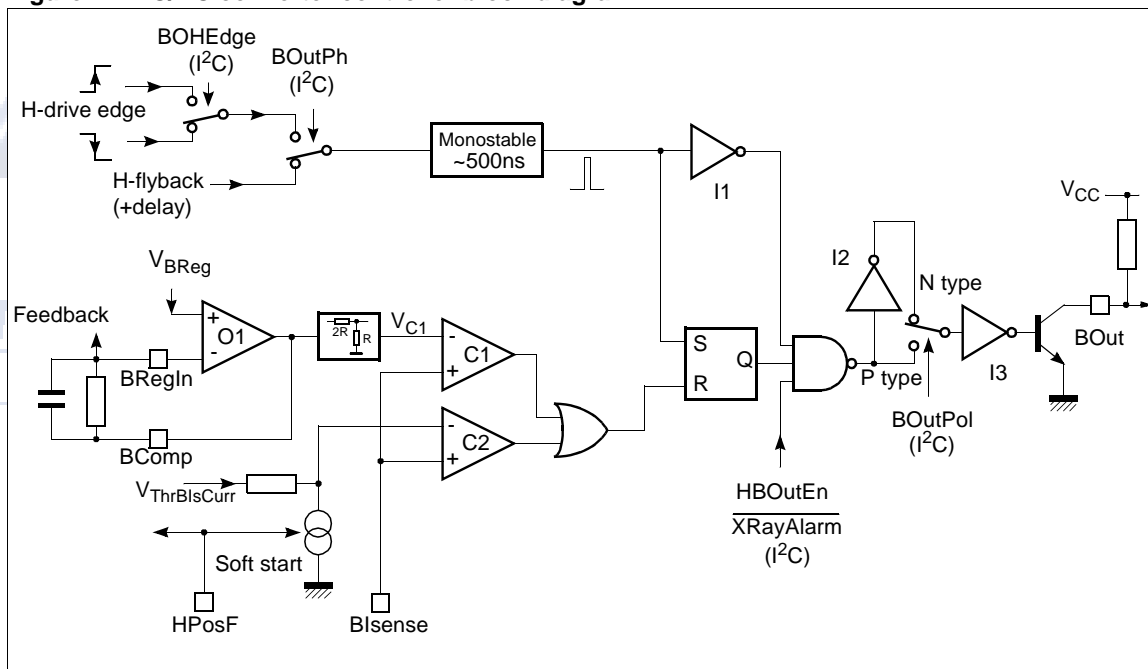
Figure 14. DC/DC converter controller block diagram
