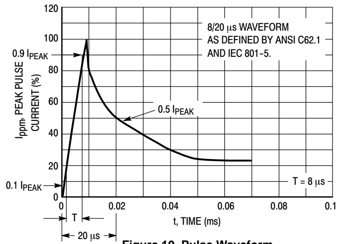
Figure 10. Pulse Waveform
