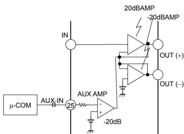
Figure 5 AUX IN
