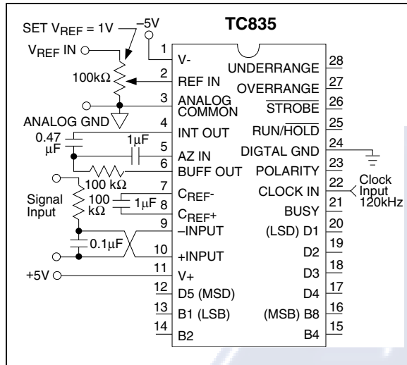
FIGURE 6-5: TEST CIRCUIT
