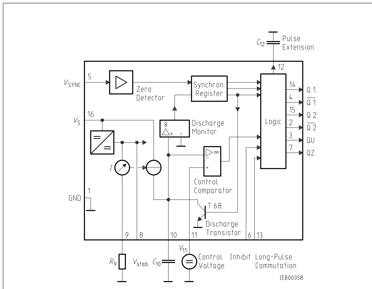
Block Diagram
