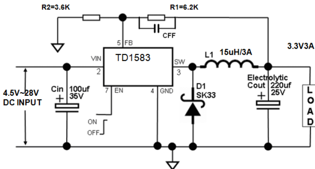
Fig9. TD1583 Typical Application Circuit @ 3.3V/3A
