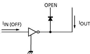
4. I_{IN(OFF)}
