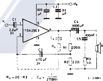
Figure 16. Typical application circuit
