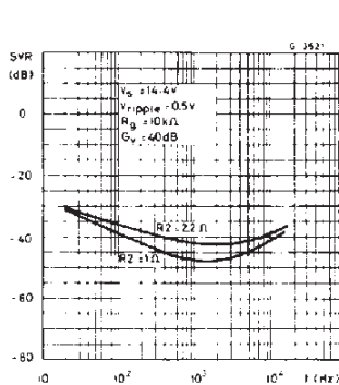
Figure 10. Supply voltage rejection vs. frequency
