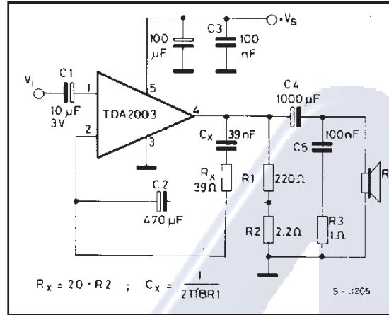
AC TEST CIRCUIT
