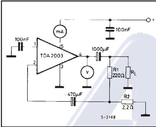
DC TEST CIRCUIT
