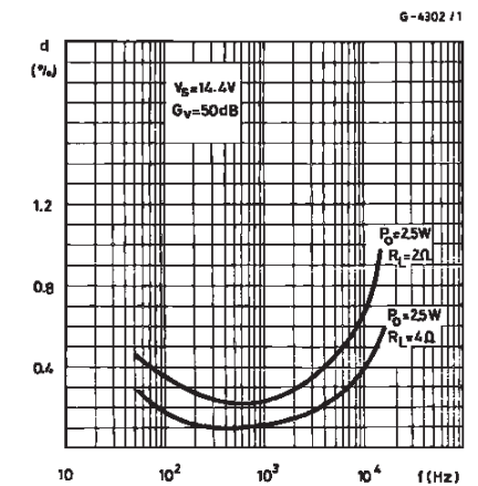
Figure 13 : Distortion versus Frequency (Stereo amplifier)
