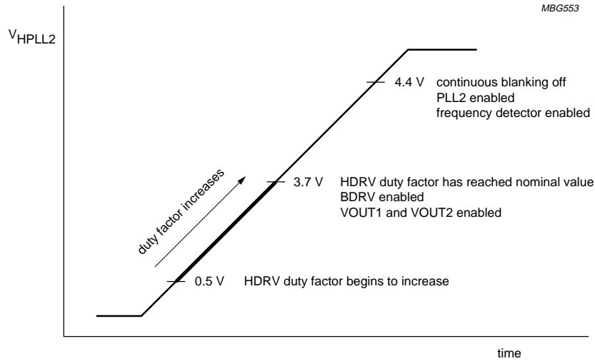
a. PLL2 start-up sequence.
