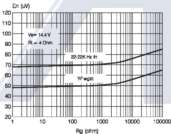
Figure 11: Output Noise vs. Source Resistance
