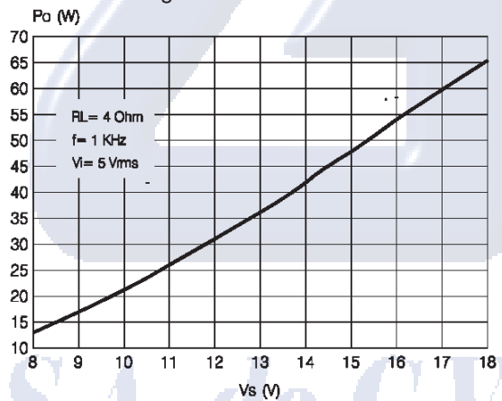
Figure 6: Maximum Output Power vs. Supply Voltage
