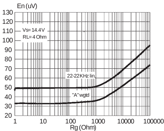
Figure 13. Output noise vs. source resistance.
