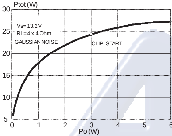
Figure 15. Power dissipation vs. output power (Music/Speech Simulation)
