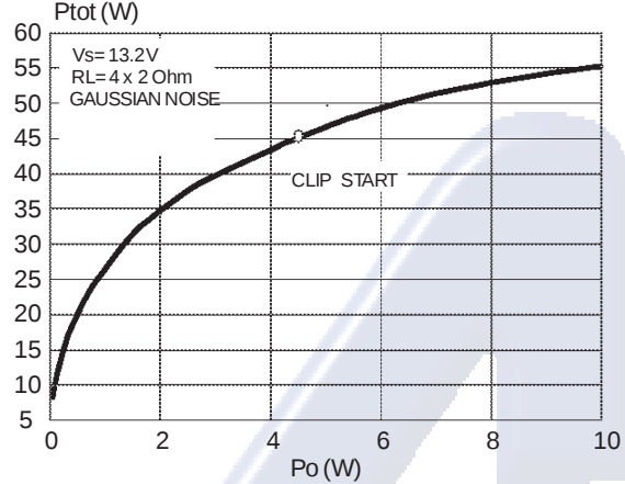
Figure 16. Power dissipation vs. output power (Music/Speech Simulation)
