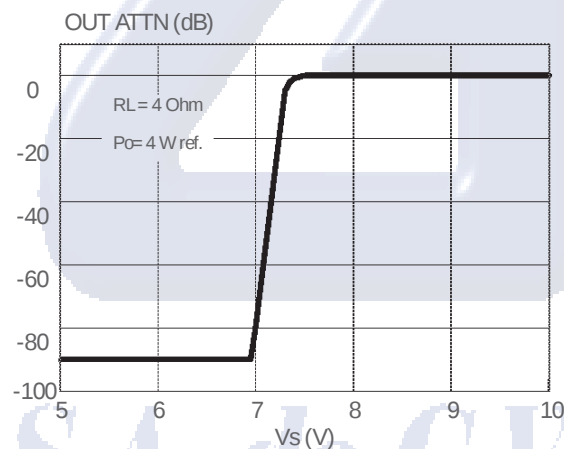
Figure 12. Output attenuation vs. supply voltage.
