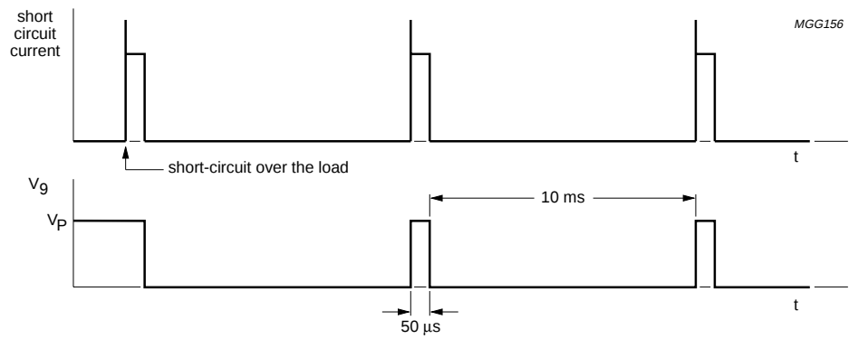
Fig.5 Short-circuit waveform.
