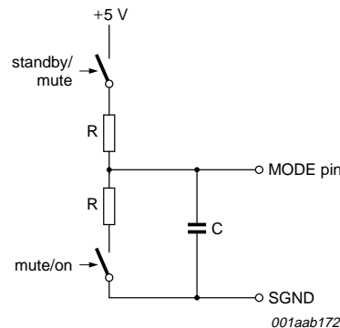
Fig 4. Example of mode selection circuit.
