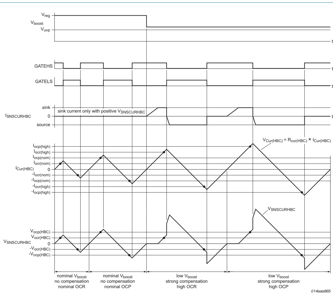
Fig 15. Boost voltage compensation
