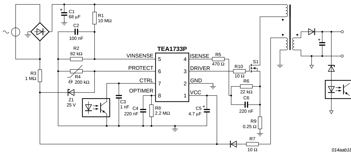
Fig 10. Typical application
