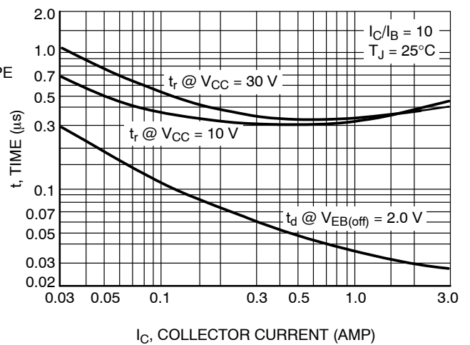
Figure 4. Turn-On Time
