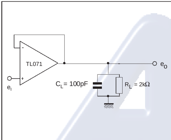
Figure 1 : Voltage Follower
