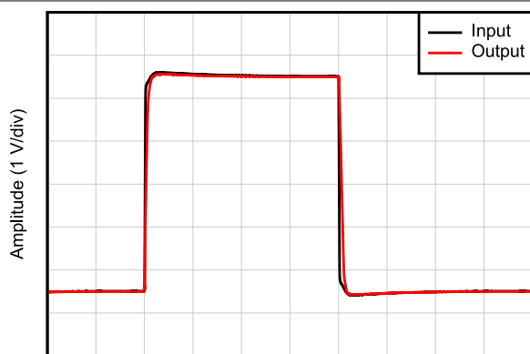
Time (2.5 \mu\text{s}/\text{div} ) C_L = 20\text{ pF} , G = 1
