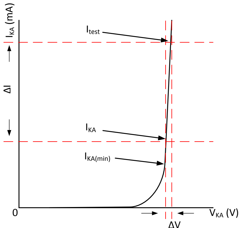
Figure 8-4. Dynamic Impedance
