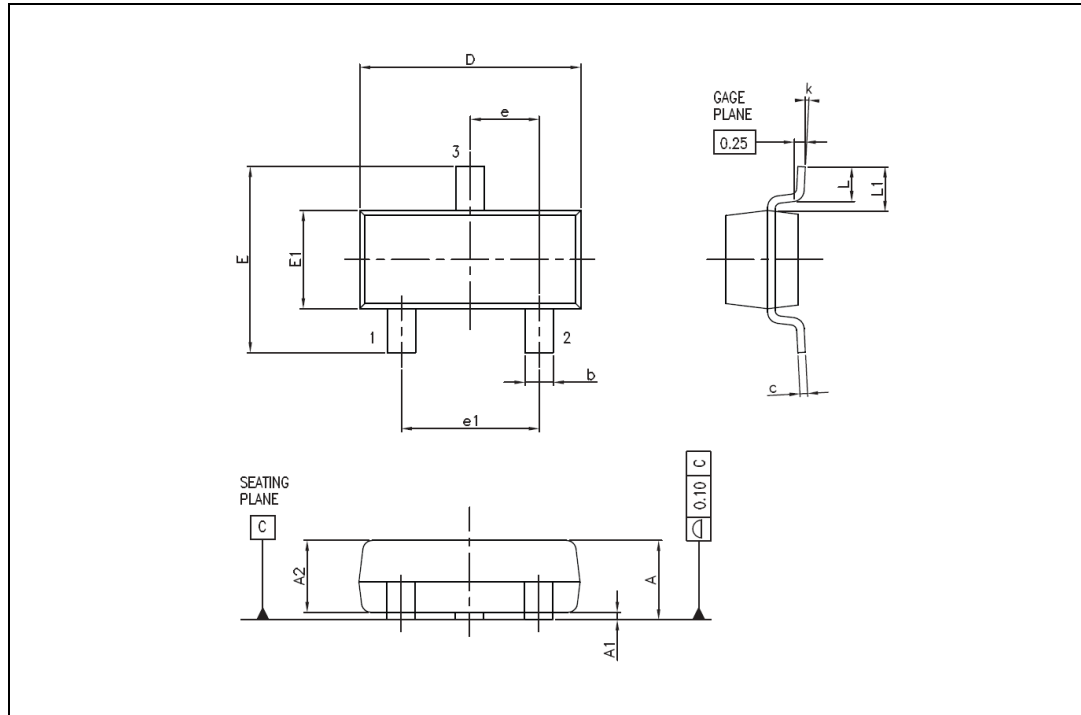
Figure 27. SOT23-3 package outline
