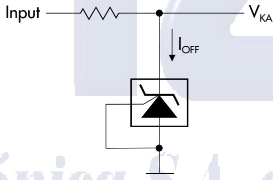
FIGURE 10 — TEST CIRCUIT FOR I_{OFF}
