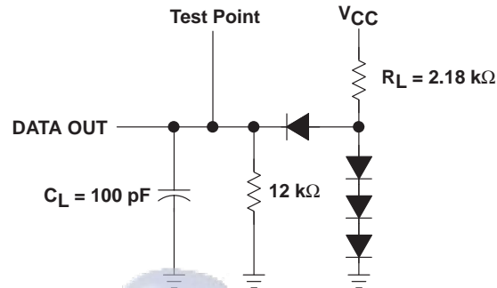
Figure 2. Load Circuit
