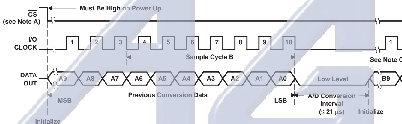
Figure 7. Timing for 10-Clock Transfer Not Using \overline{\text{CS}}
