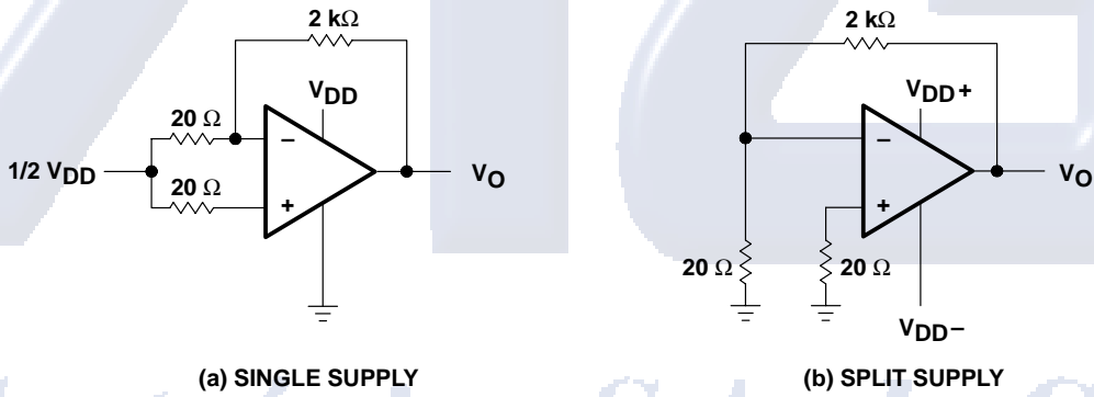
Figure 2. Noise-Test Circuit
