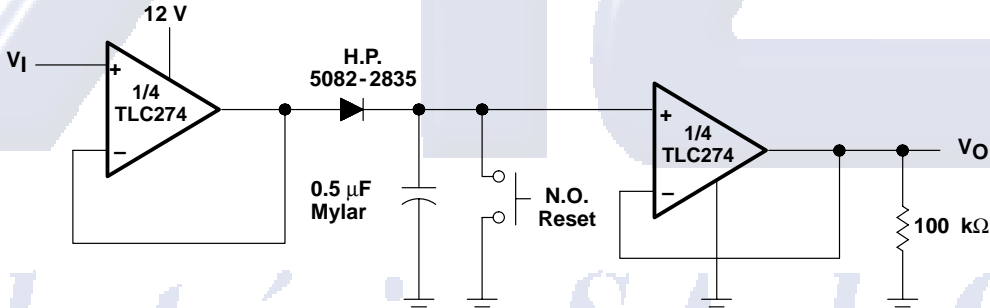
Figure 45. Positive-Peak Detector
