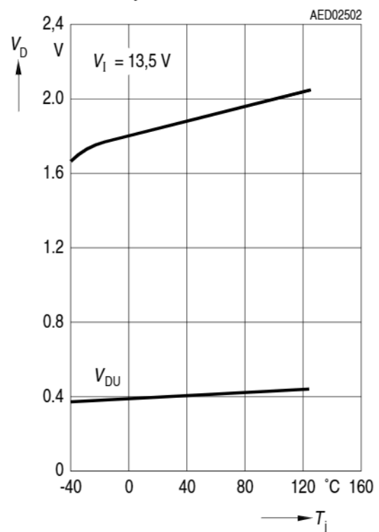
Switching Voltage V_{\text{DU}} , V_{\text{DL}} versus Temperature T_j
