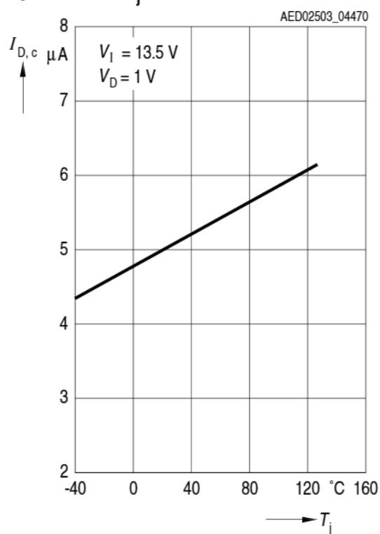
Charge Current I_{D,c} versus Temperature T_j
