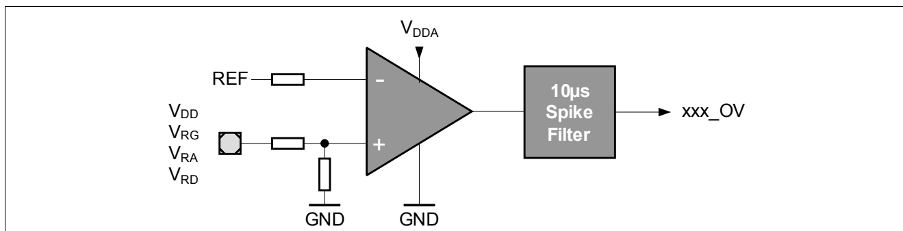
Figure 4-22 Overvoltage comparator
