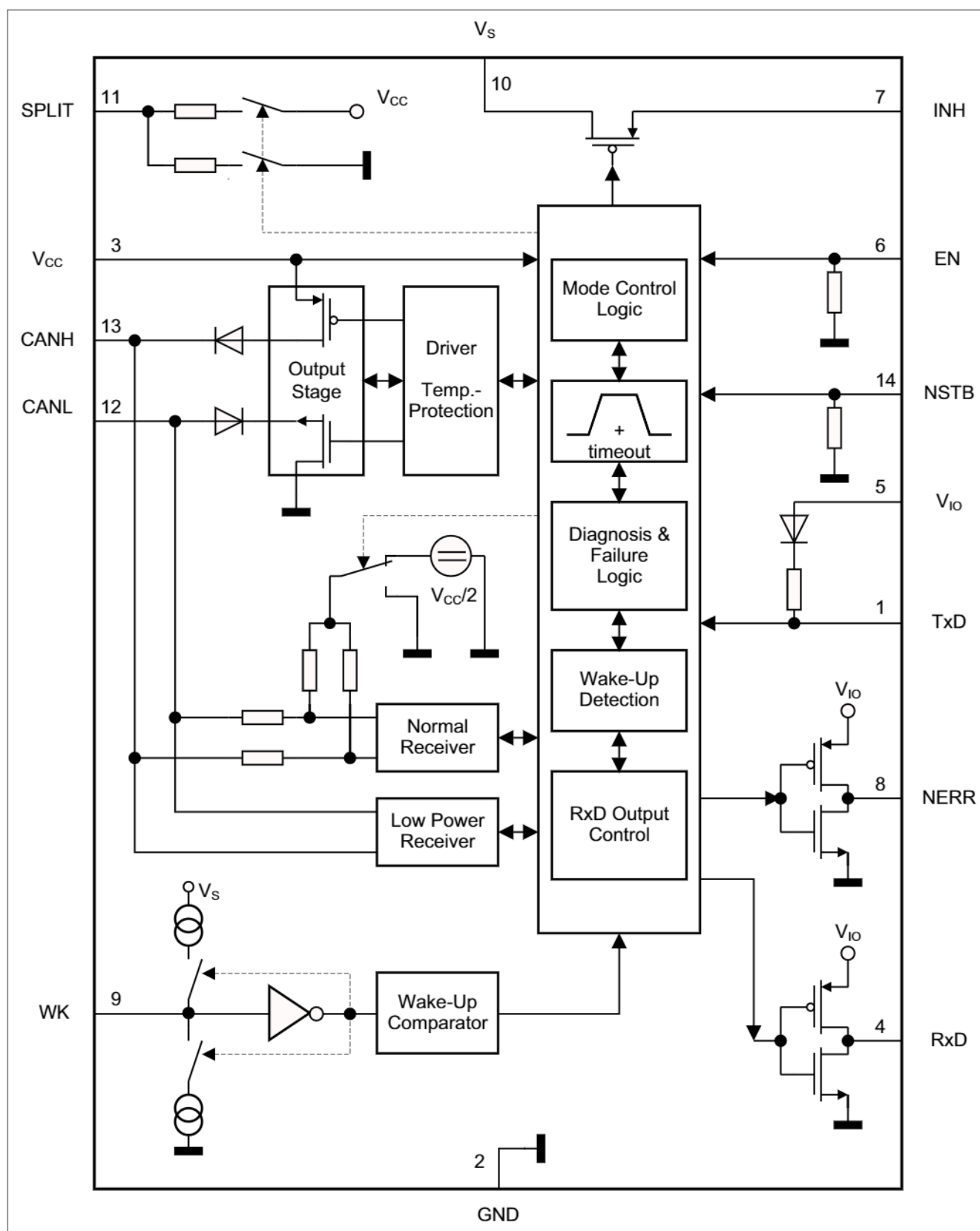
Figure 1 Block Diagram
