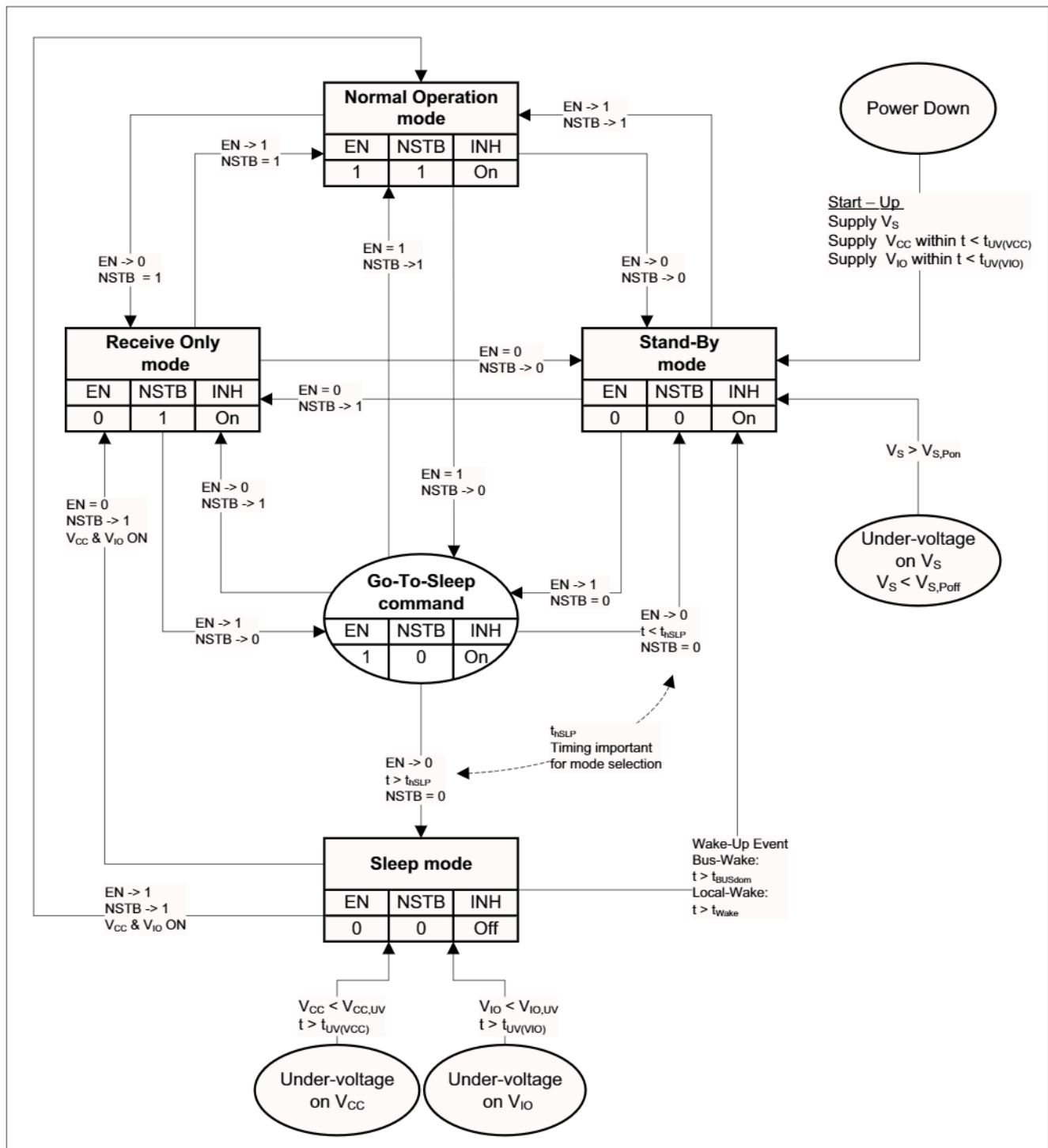
Figure 4 Operation Modes
