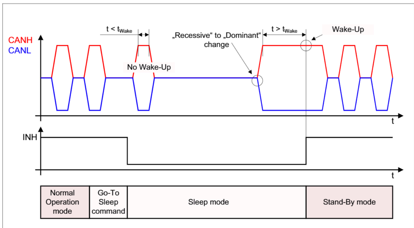
Figure 6 Remote Wake-Up
