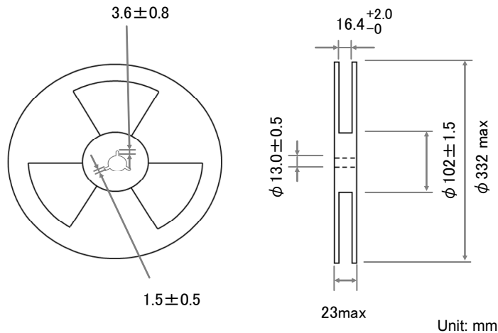
Figure 4 Reel Forms
