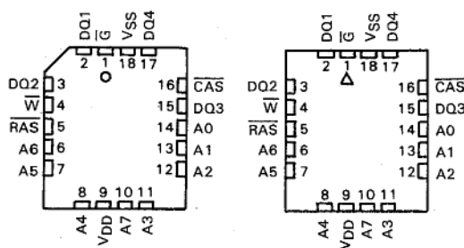
TMS4416 ... FPL PACKAGE (TOP VIEW) SMJ4416 ... FG PACKAGE (TOP VIEW)
