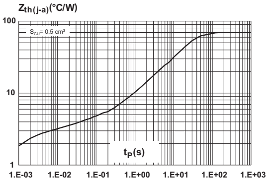
Figure 4. Thermal impedance junction to ambient versus pulse duration, PCB FR4, copper thickness 35 \mu\text{m}
