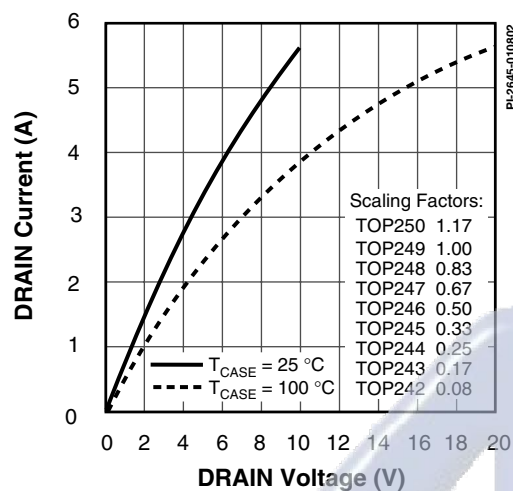
Figure 67. Output Characteristics.
