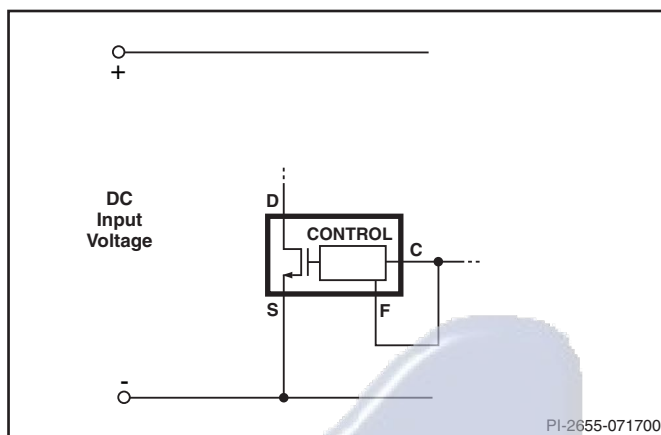
Figure 15. Half Frequency Operation (66 kHz).
