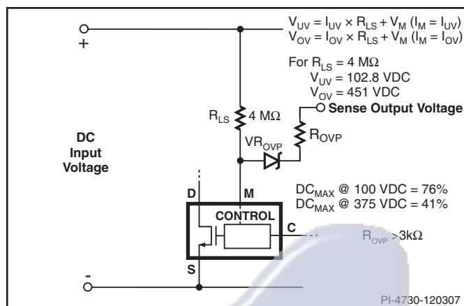
Figure 32. Line Sensing for Undervoltage, Overvoltage, Line Feed-Forward and Hysteretic Output Overvoltage Protection.
