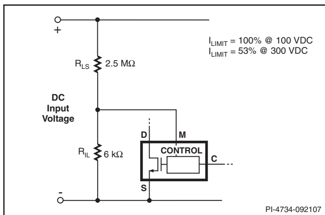
Figure 36. Current Limit Reduction with Line Voltage (Not Normally Required – See M Pin Operation Description).
