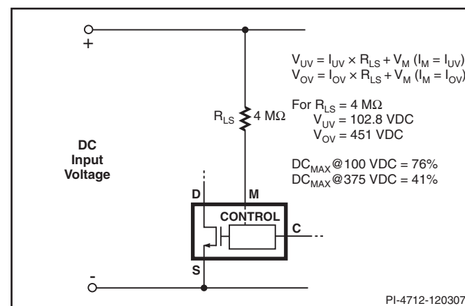
Figure 7. P/G Package Line Sense.
