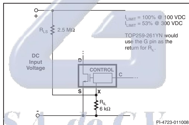
Figure 23. Current Limit Reduction with Line Voltage.
