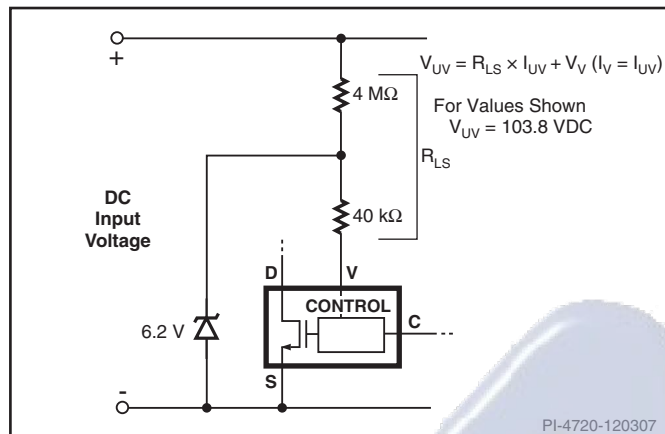
Figure 20. Line Sensing for Undervoltage Only (Overvoltage Disabled).
