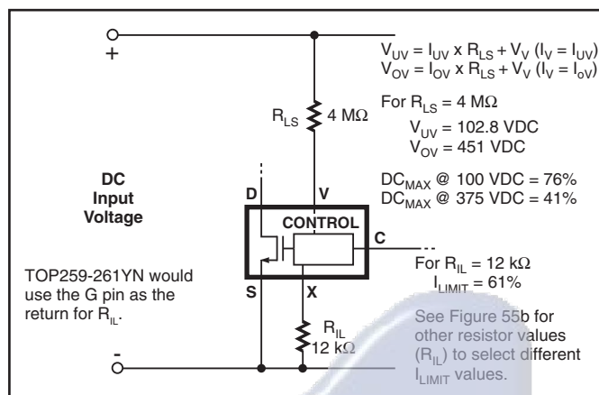
Figure 27. Line Sensing and Externally Set Current Limit.
