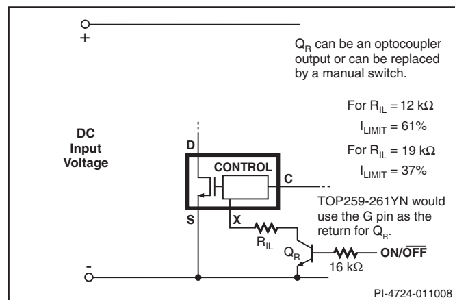
Figure 25. Active-on Remote ON/OFF with Externally Set Current Limit.
