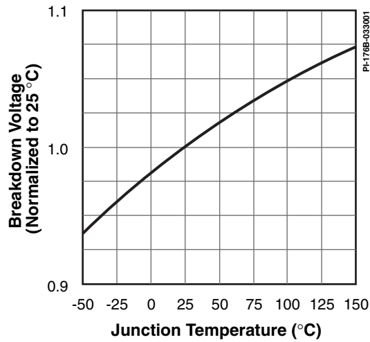
Figure 36. Breakdown Voltage vs. Temperature.
