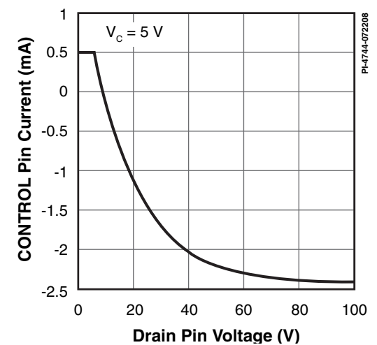
Figure 47. I_c vs. DRAIN Voltage.
