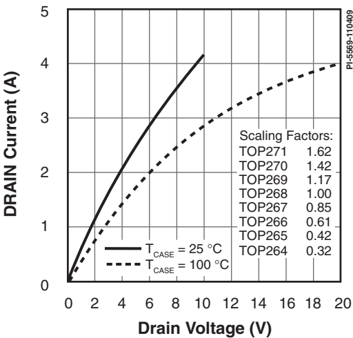
Figure 46. Output Characteristics.
