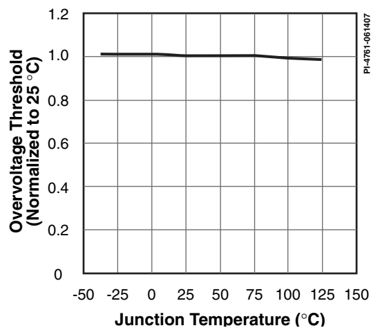
Figure 40. Overvoltage Threshold vs. Temperature.
