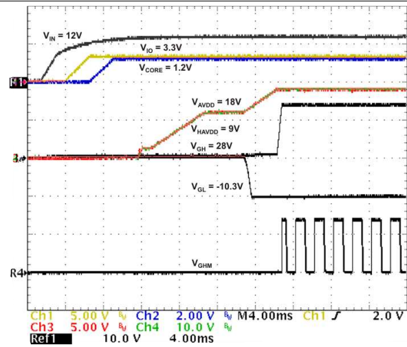
Figure 21. Startup Sequencing V_{(GL)} Driven By Boost
