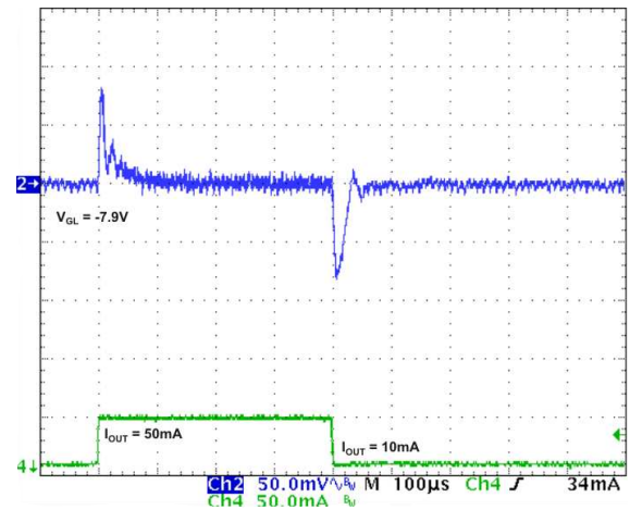
Figure 45. Negative CP ( V_{GL} ) Load Transient Response
