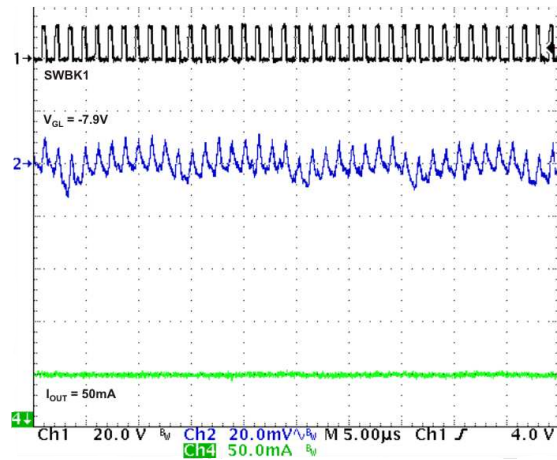
Figure 44. Negative Charge-Pump ( V_{GL} ) Normal Load
