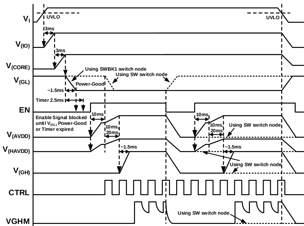
Figure 11. TPS65177A Power-up Sequencing
