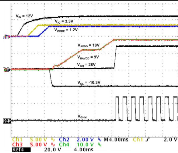
Figure 20. Startup Sequencing V_{(GL)} Driven By Buck 1
