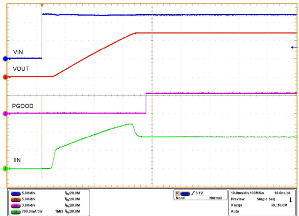
Figure 9-4. Hot-Plug Start-Up With Load on Output, dVdt Limited
