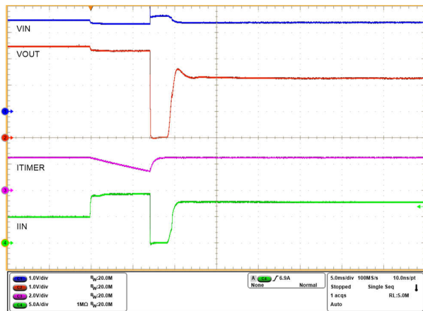
Figure 9-15. Circuit Breaker With Transient Overcurrent Blanking Interval of 6 ms; Device Restarts in Current Limit Mode
