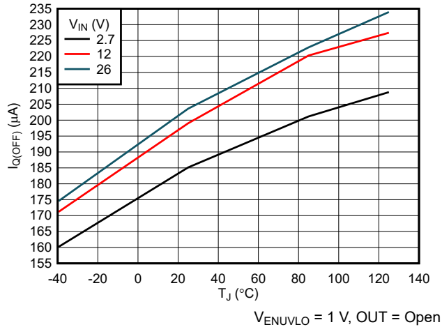
Figure 7-7. Shut-Down Current vs Temperature
