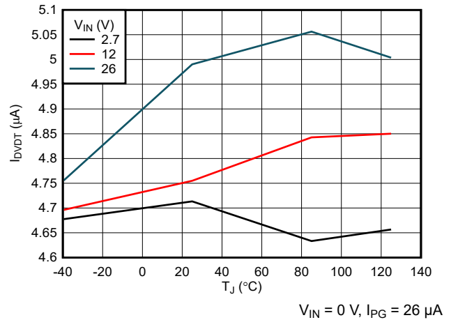
Figure 7-14. DVDVT Pin Charging Current vs Temperature
