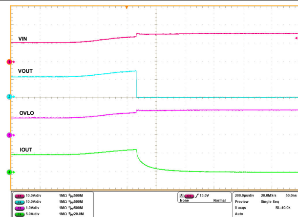
Figure 7-24. Overvoltage Protection
