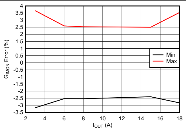
Figure 7-12. Output Current Monitor Gain ( G_{IMON} ) Accuracy
