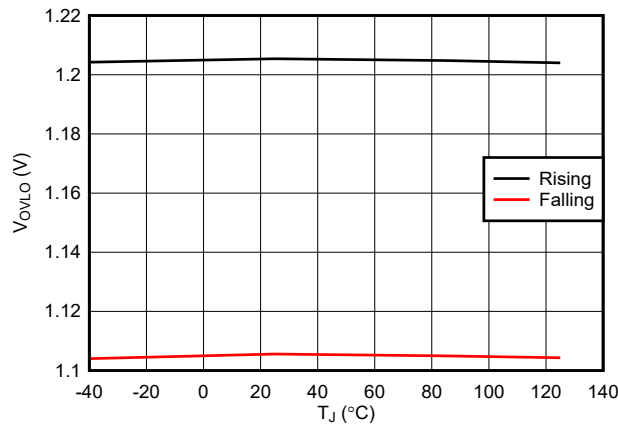
Figure 7-3. OVLO Pin Threshold vs Temperature
