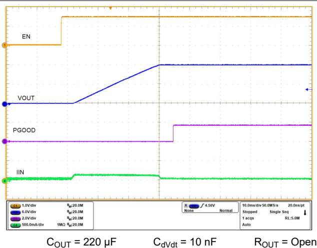
Figure 7-22. Startup With EN - dVdt Limited
