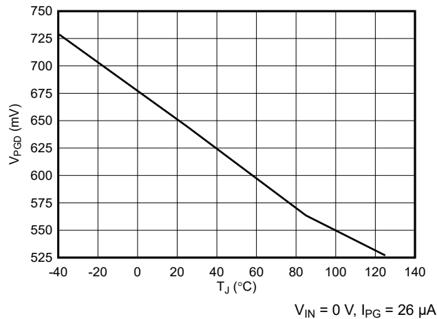
Figure 7-15. Power Good Output Voltage (De-asserted State) vs Temperature
