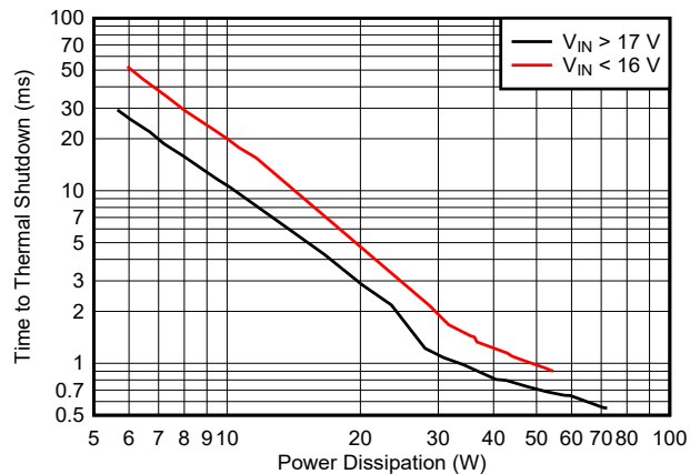
Figure 7-20. Thermal Shutdown Plot - Inrush/Overload
