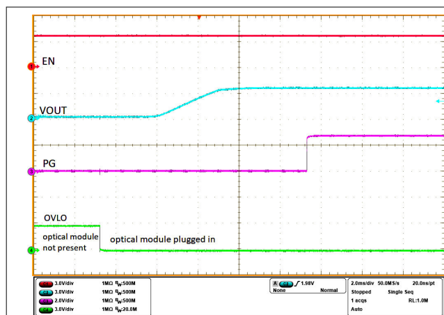
Figure 9-13. Output Voltage Profile When Optical Module is Inserted
