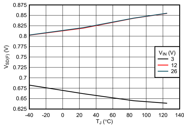
Figure 7-5. EN/UVLO Falling Threshold for Lowest Current Consumption
