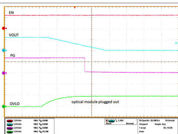
Figure 9-14. Output Voltage Profile When Optical Module is Plugged Out
