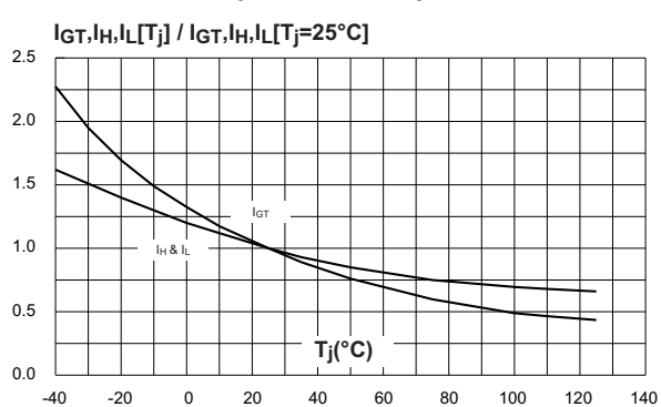
Figure 4. Relative variation of gate trigger current, holding current and latching current versus junction temperature
