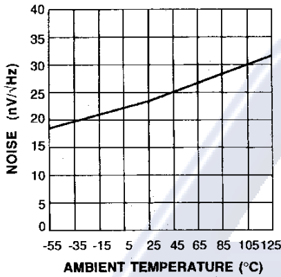
EQUIVALENT INPUT NOISE vs AMBIENT TEMPERATURE
