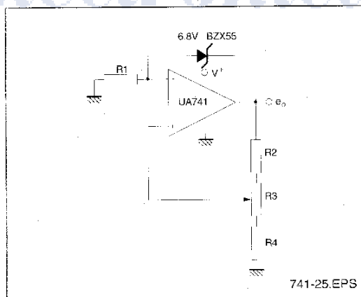
POSITIVE VOLTAGE REFERENCE
