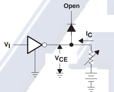
Figure 4. V_{I(on)} Test Circuit
