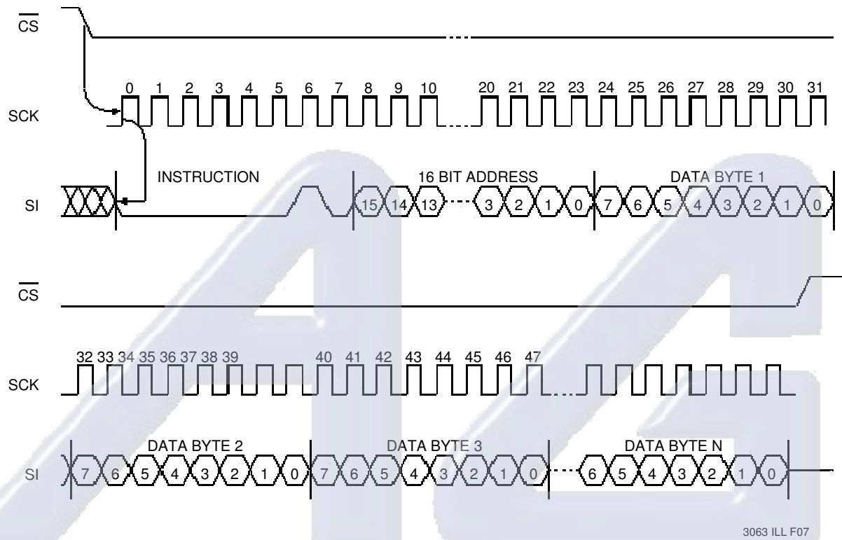
Figure 5. Page Write Operation Sequence
