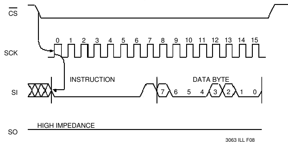
Figure 6. Write Status Register Operation Sequence
