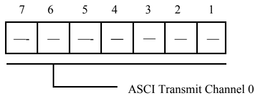
Figure 28. ASCI Register Channel 0
