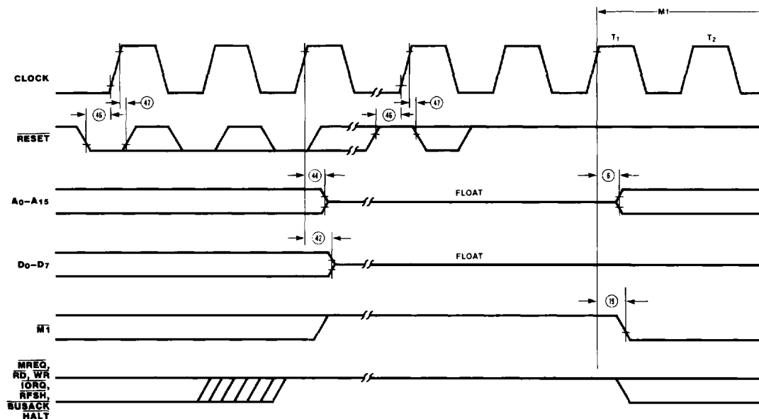
Figure 9. Reset Cycle
