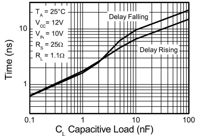
Propagation Delay
