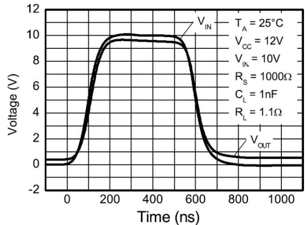
Switching Speed
