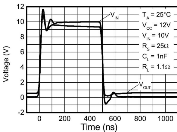
Switching Speed
